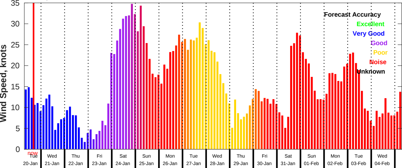
GFS Wind Speed Forecast for NDBC 41004 from 20-Jan-2026 07:00:00 to 05-Feb-2026 07:00:00
