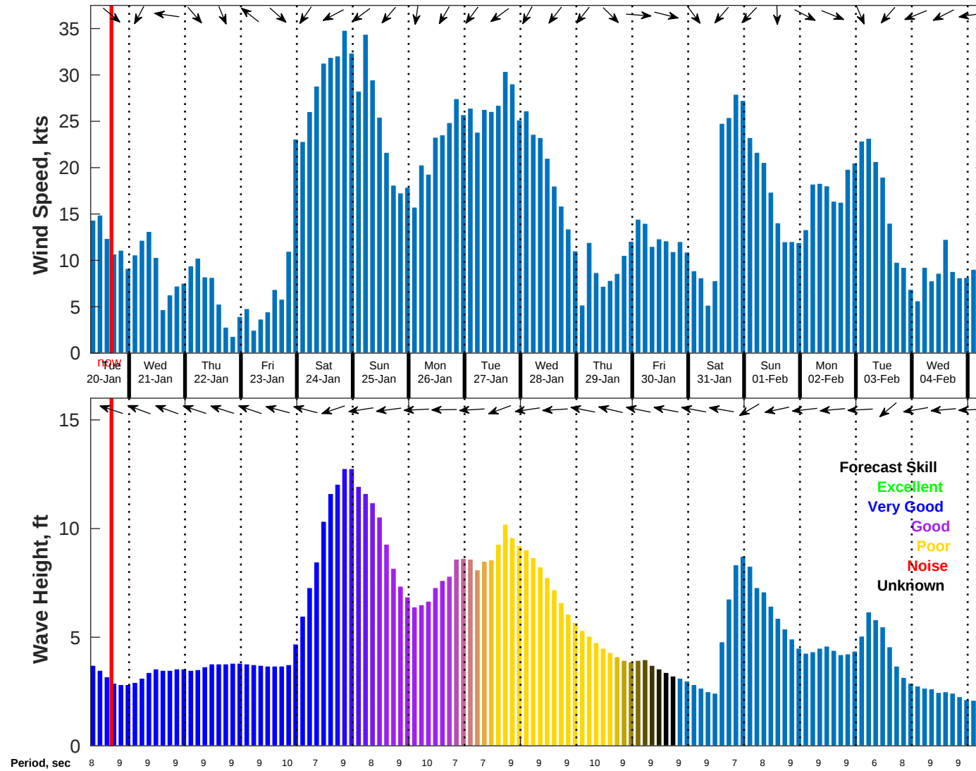
Wind & Wave Forecast for NDBC 41004 from 20-Jan-2026 07:00:00 to 05-Feb-2026 07:00:00
