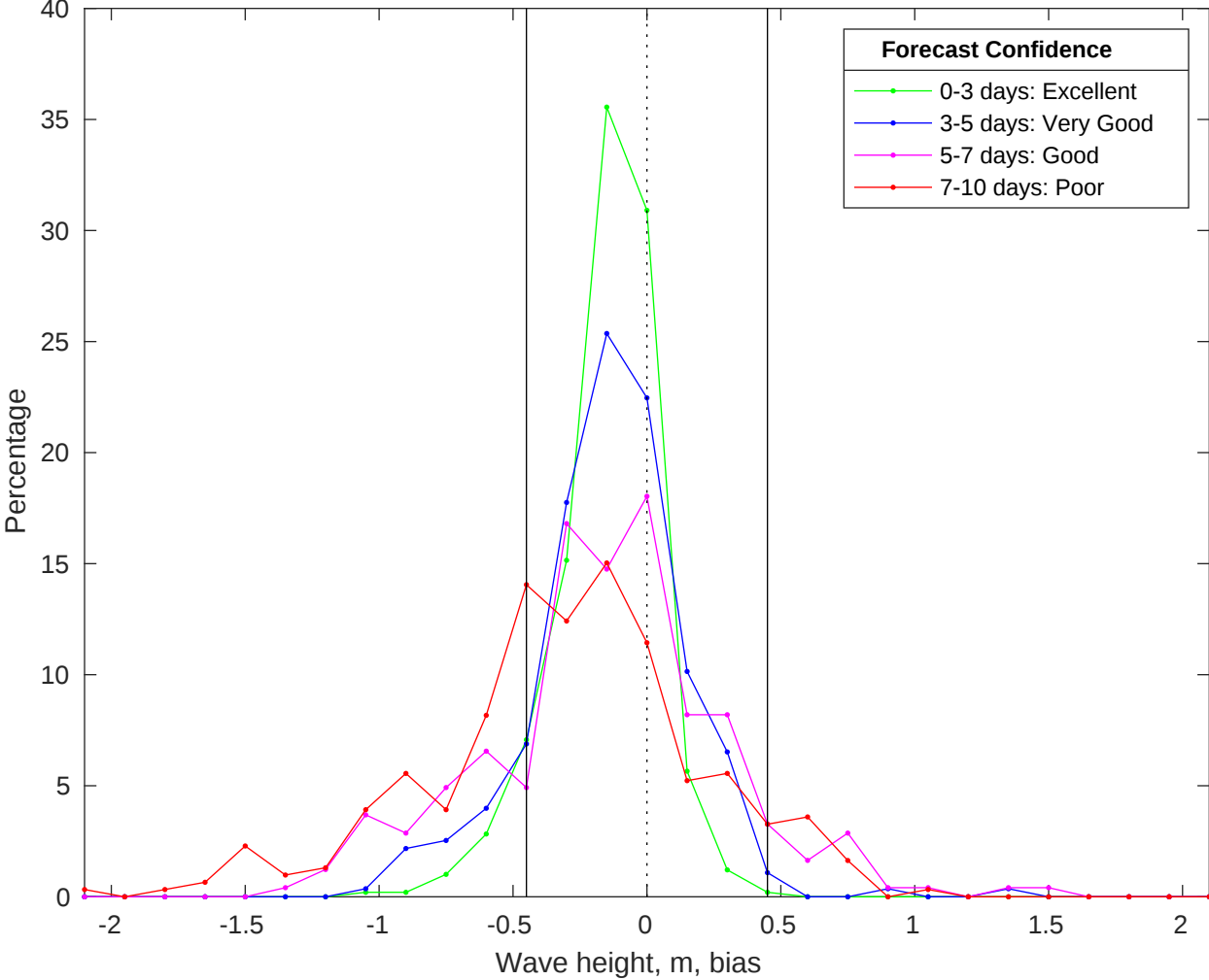
NDBC 41013 vs CMEMS Waves Bias Histogram: 20-Jan-2026
