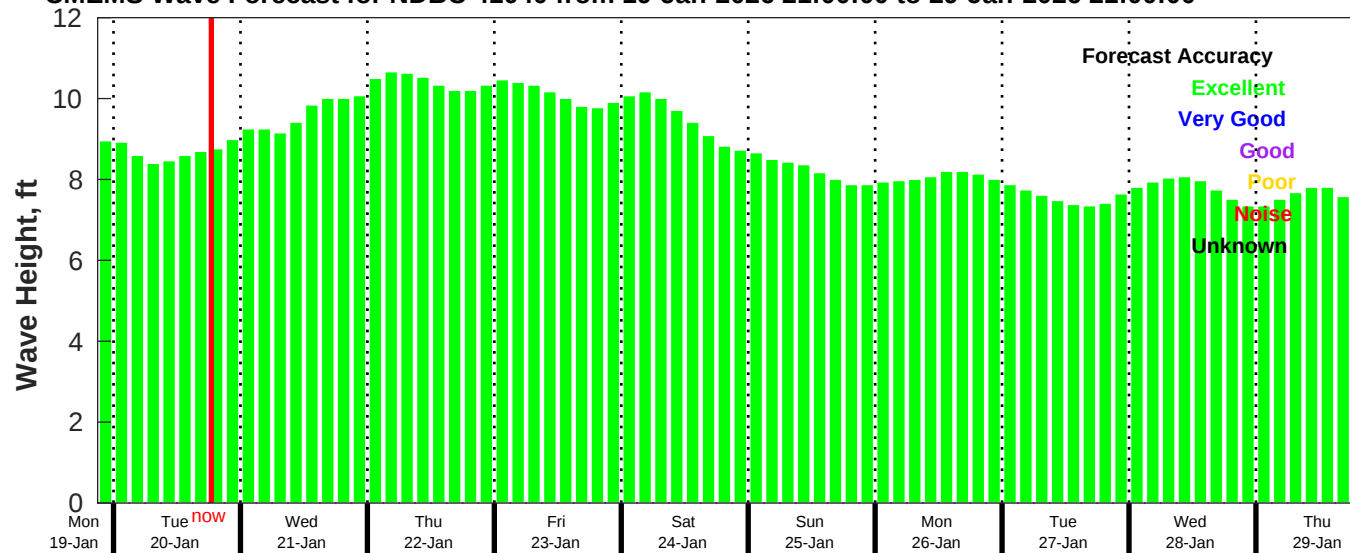
CMEMS Wave Forecast for NDBC 41040 from 19-Jan-2026 21:00:00 to 29-Jan-2026 21:00:00
