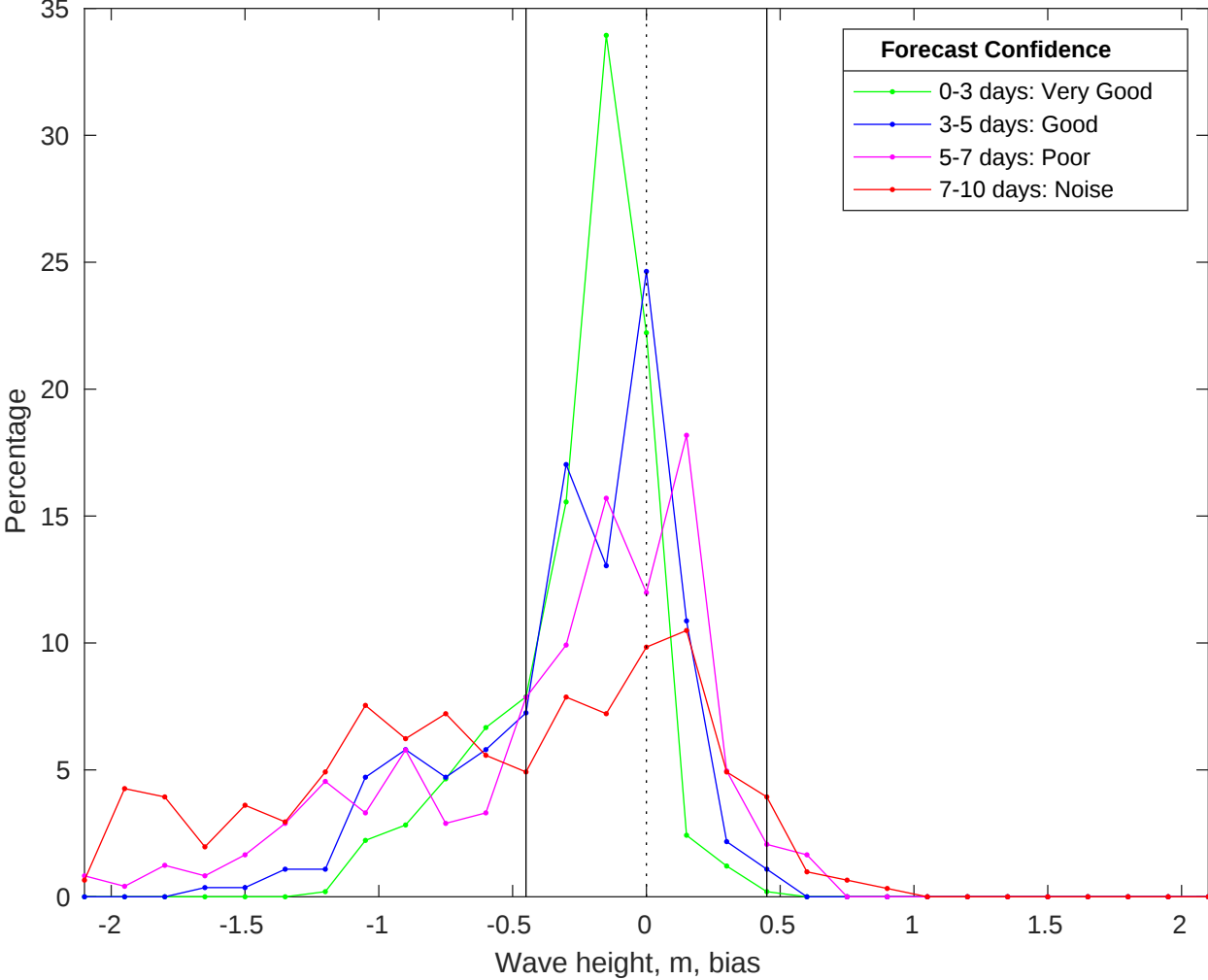
NDBC 42019 vs CMEMS Waves Bias Histogram: 20-Jan-2026
