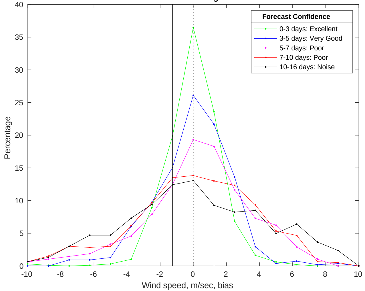
NDBC 42019 vs GFS Winds Bias Histogram: 20-Jan-2026
