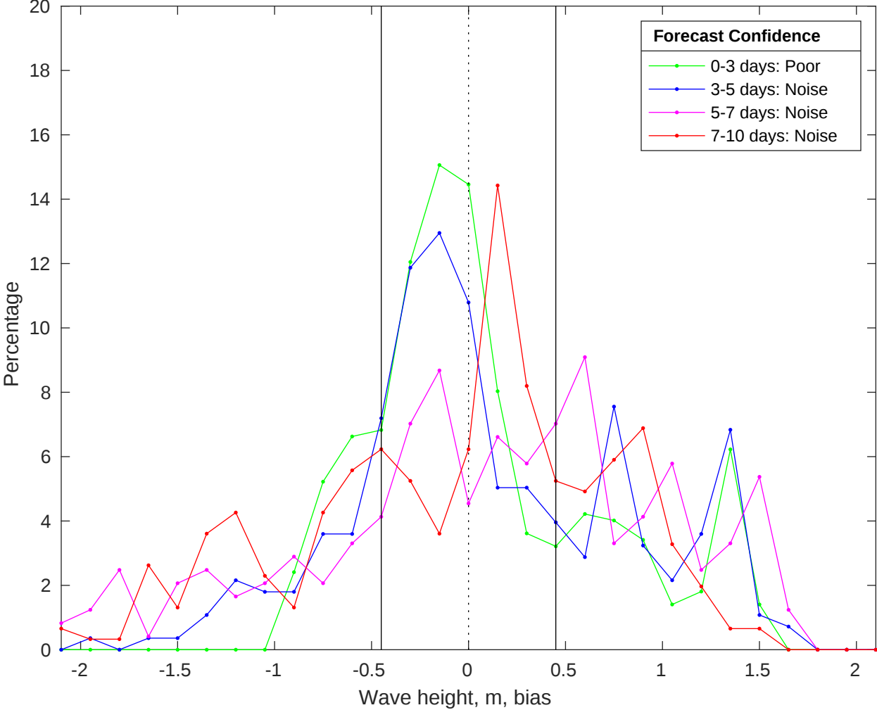
NDBC 42020 vs CMEMS Waves Bias Histogram: 20-Jan-2026
