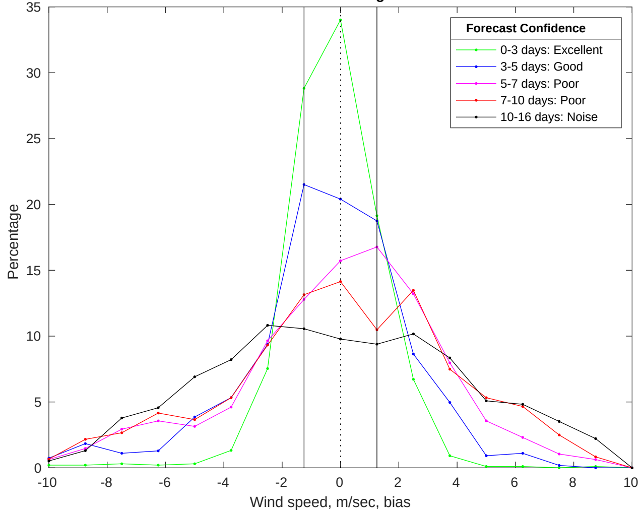
NDBC 42020 vs GFS Winds Bias Histogram: 20-Jan-2026
