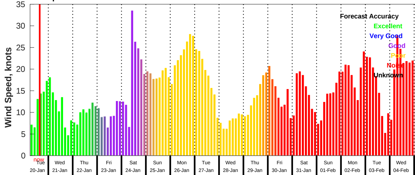
GFS Wind Speed Forecast for NDBC 42020 from 20-Jan-2026 06:00:00 to 05-Feb-2026 06:00:00
