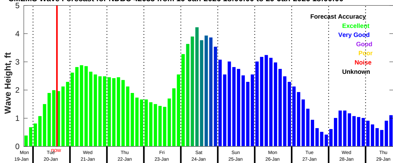
CMEMS Wave Forecast for NDBC 42035 from 19-Jan-2026 18:00:00 to 29-Jan-2026 18:00:00
