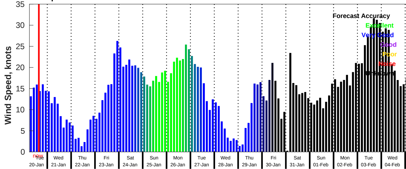
GFS Wind Speed Forecast for NDBC 42035 from 20-Jan-2026 06:00:00 to 05-Feb-2026 06:00:00
