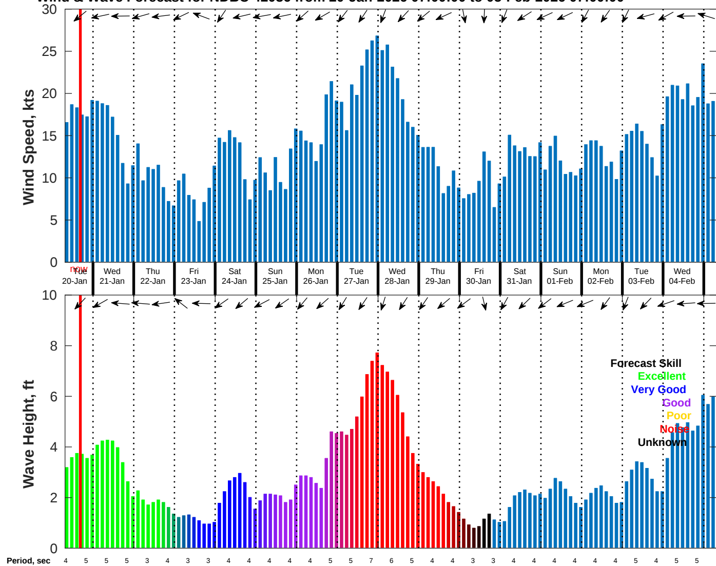
Wind & Wave Forecast for NDBC 42036 from 20-Jan-2026 07:00:00 to 05-Feb-2026 07:00:00
