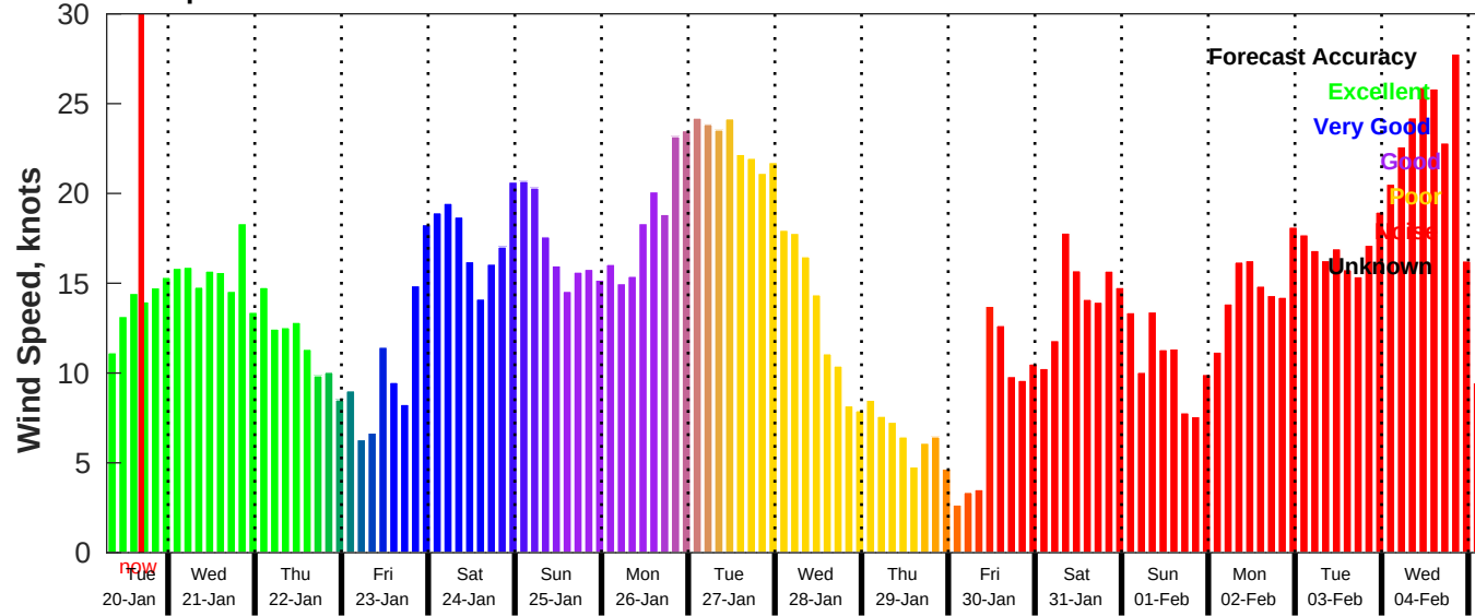
GFS Wind Speed Forecast for NDBC 42040 from 20-Jan-2026 07:00:00 to 05-Feb-2026 07:00:00
