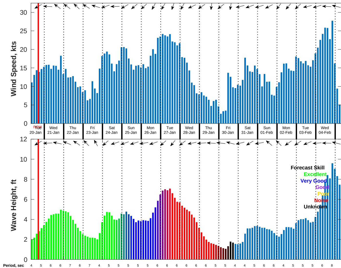
Wind & Wave Forecast for NDBC 42040 from 20-Jan-2026 07:00:00 to 05-Feb-2026 07:00:00
