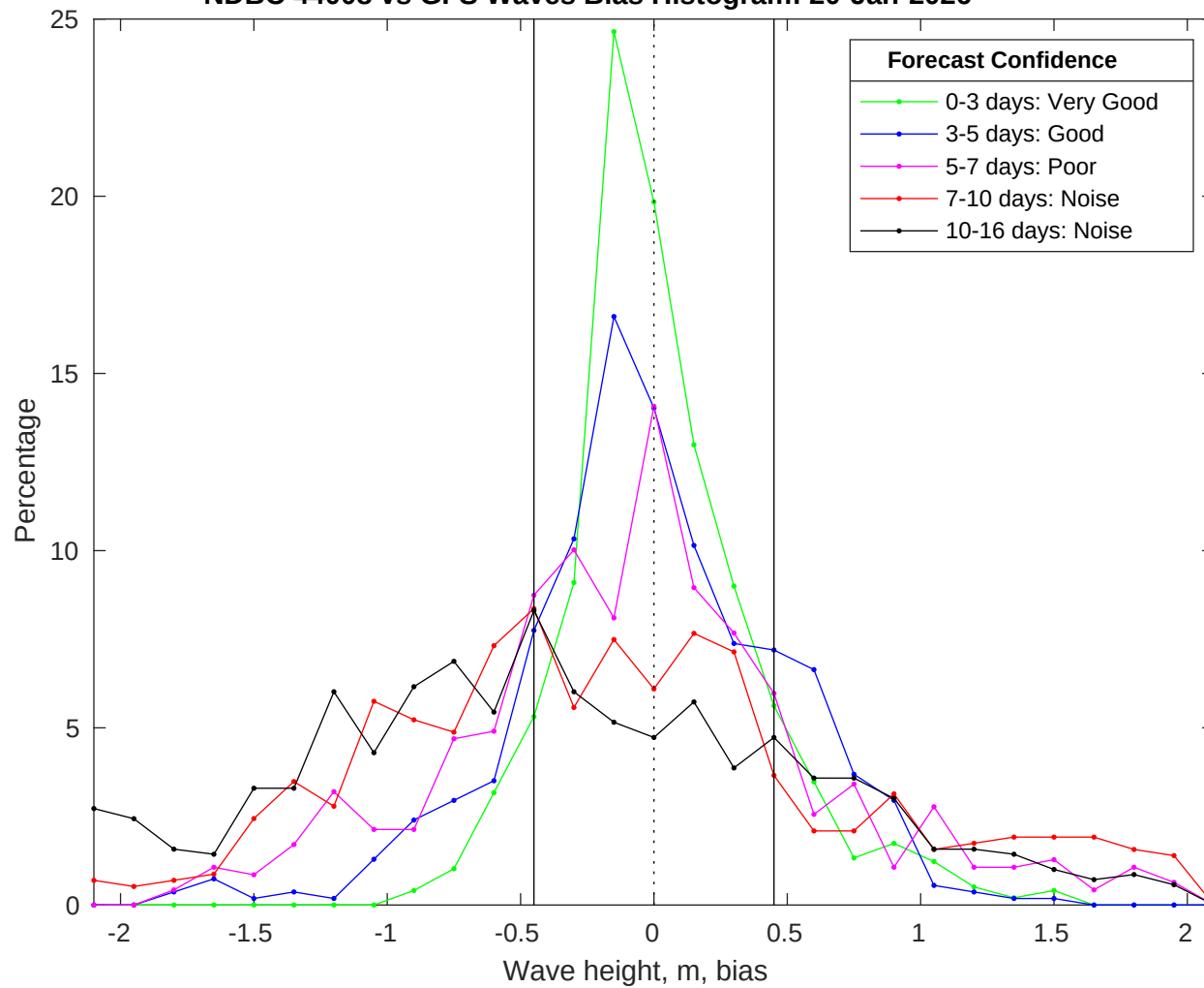
NDBC 44008 vs GFS Waves Bias Histogram: 20-Jan-2026
