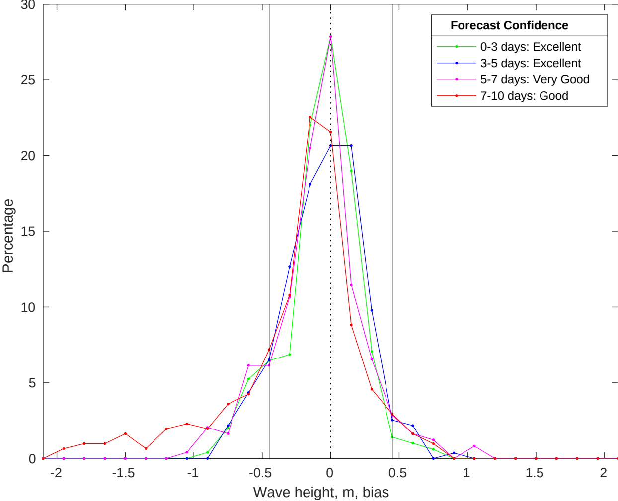
NDBC 46011 vs CMEMS Waves Bias Histogram: 20-Jan-2026
