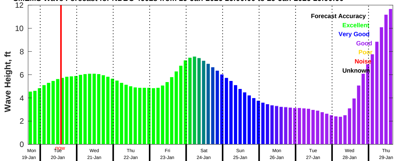
CMEMS Wave Forecast for NDBC 46028 from 19-Jan-2026 16:00:00 to 29-Jan-2026 16:00:00
