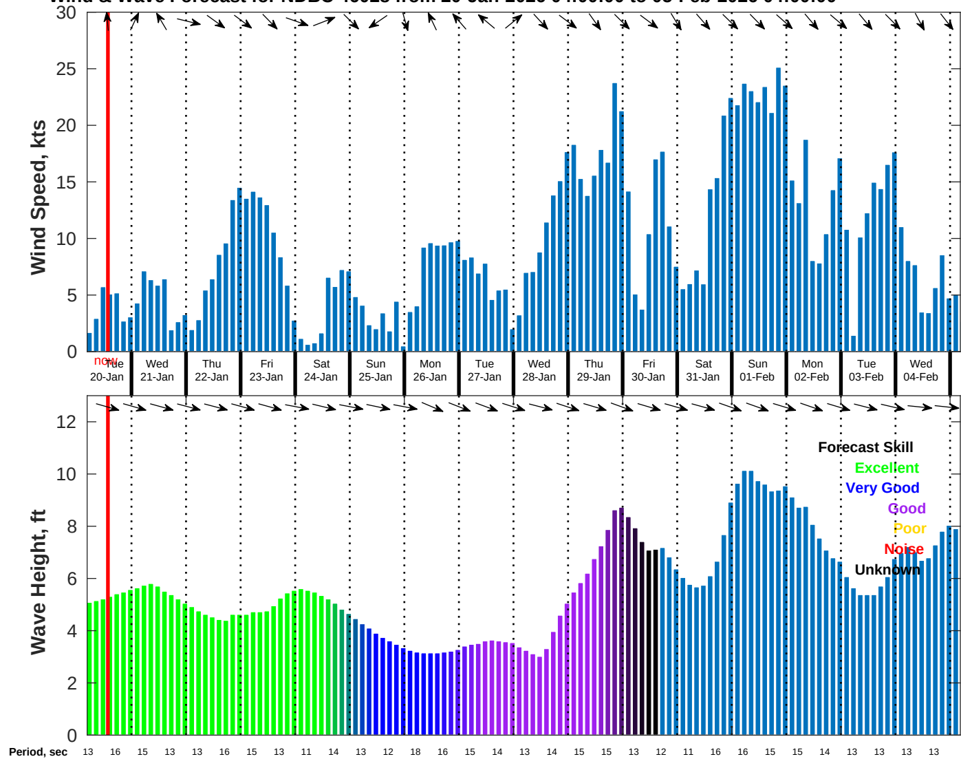
Wind & Wave Forecast for NDBC 46028 from 20-Jan-2026 04:00:00 to 05-Feb-2026 04:00:00
