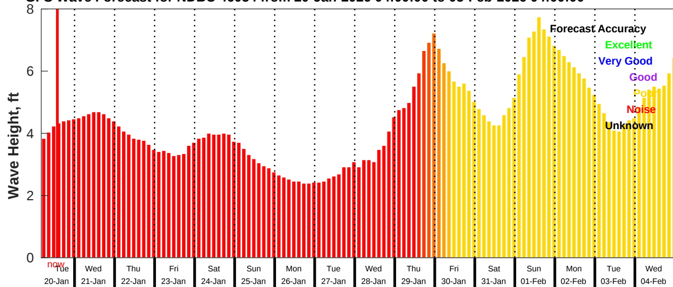
GFS Wave Forecast for NDBC 46054 from 20-Jan-2026 04:00:00 to 05-Feb-2026 04:00:00
