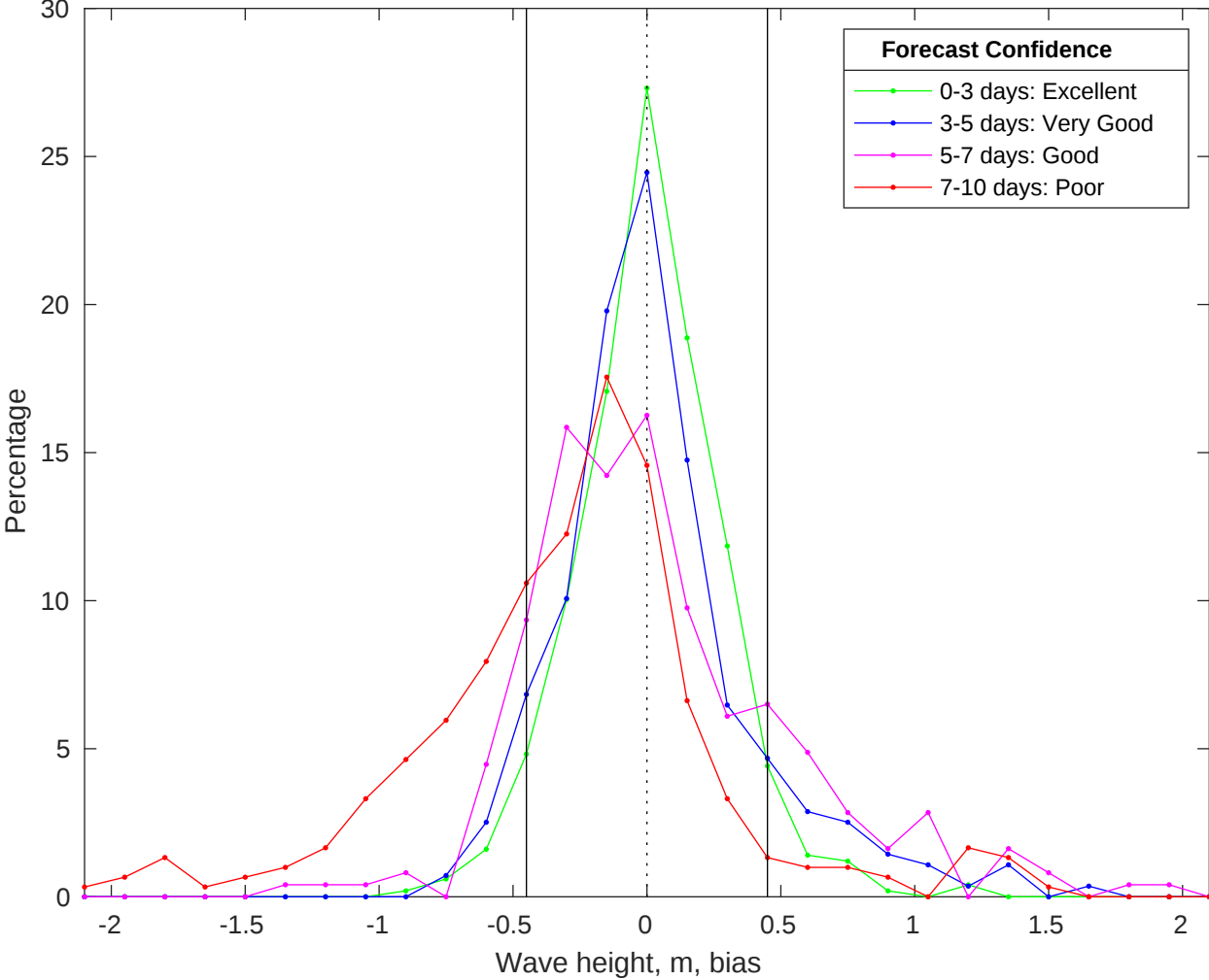
NDBC 46059 vs CMEMS Waves Bias Histogram: 20-Jan-2026
