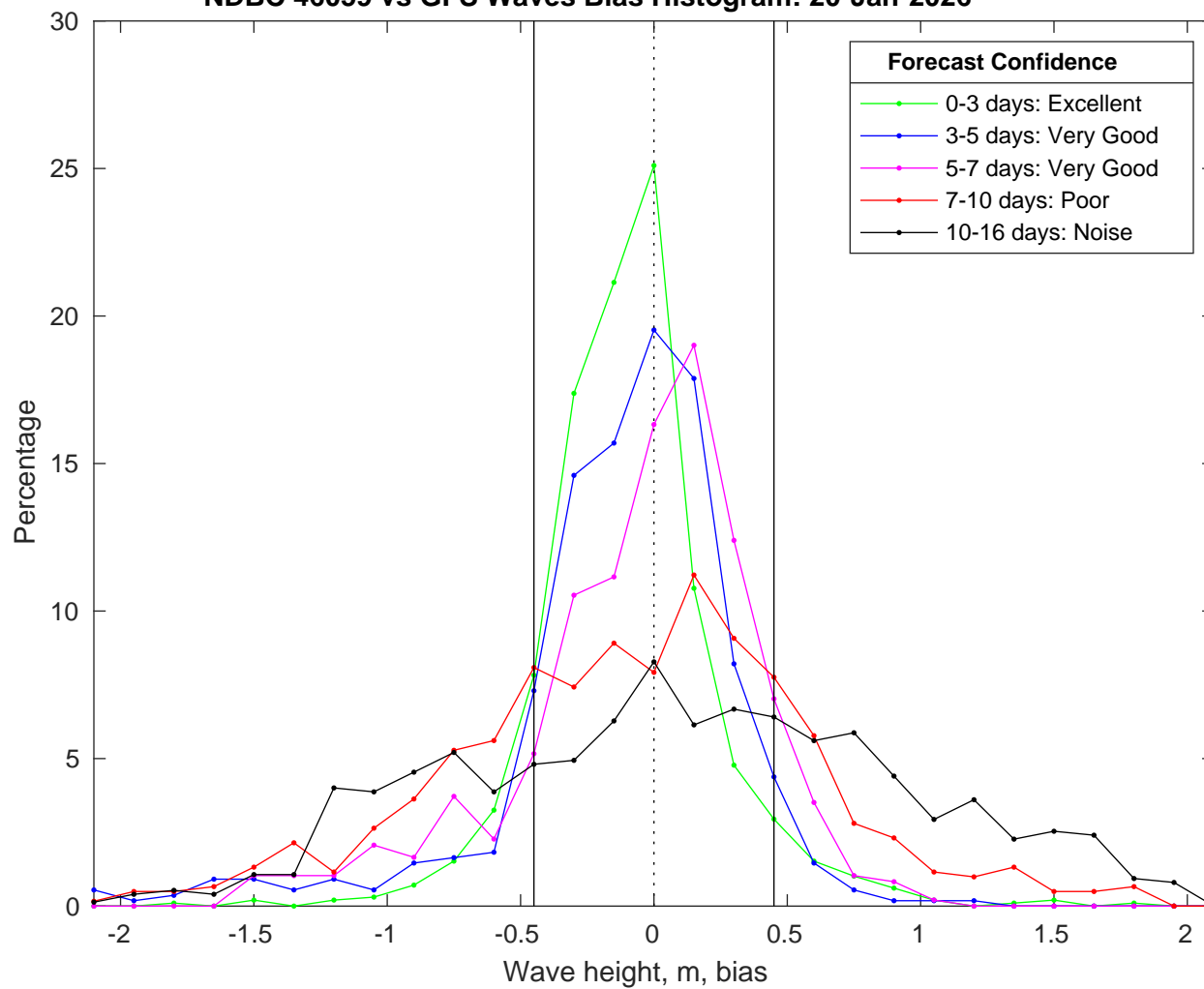
NDBC 46059 vs GFS Waves Bias Histogram: 20-Jan-2026
