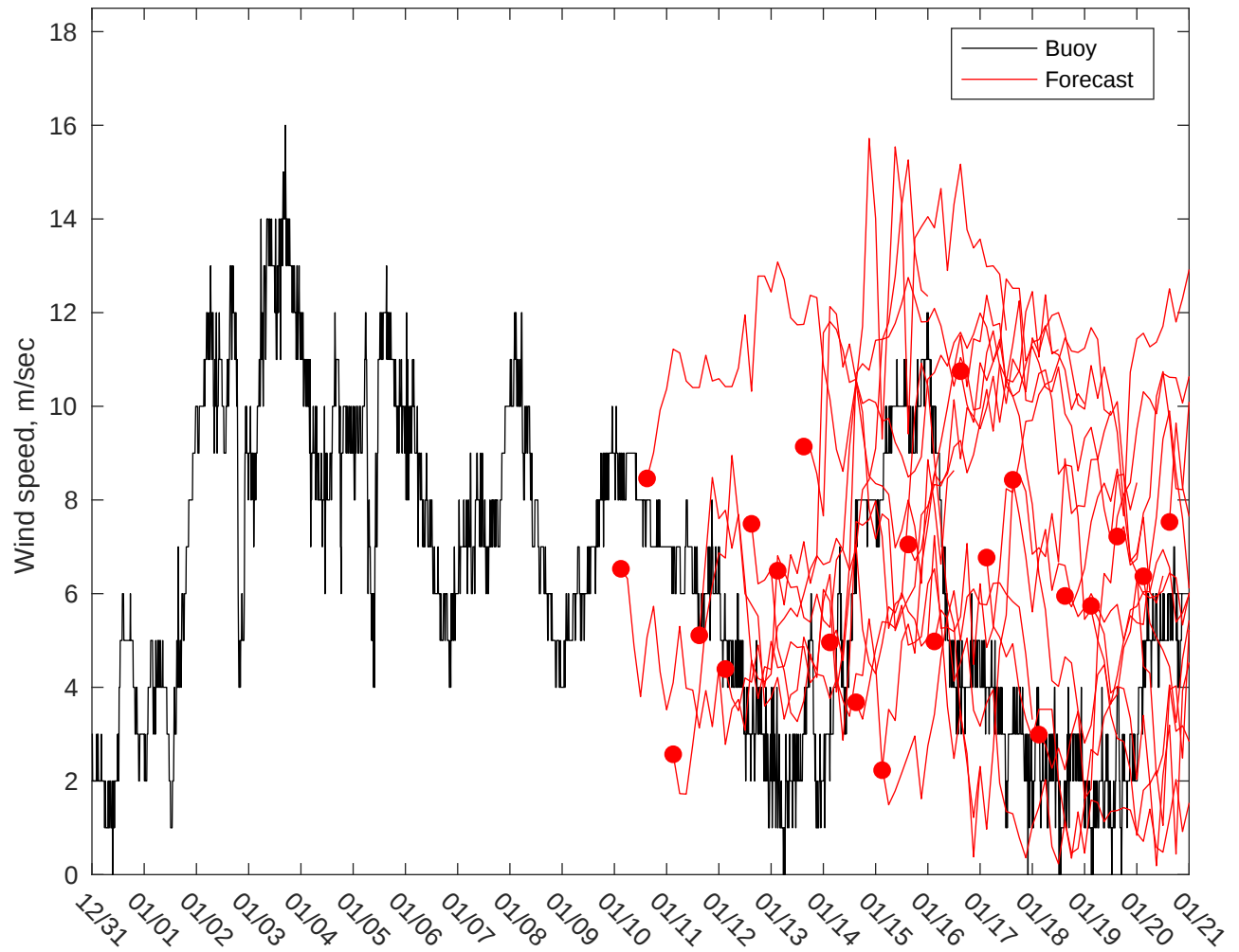
NDBC 46059 vs GFS Winds: 10 to 16 day forecast
