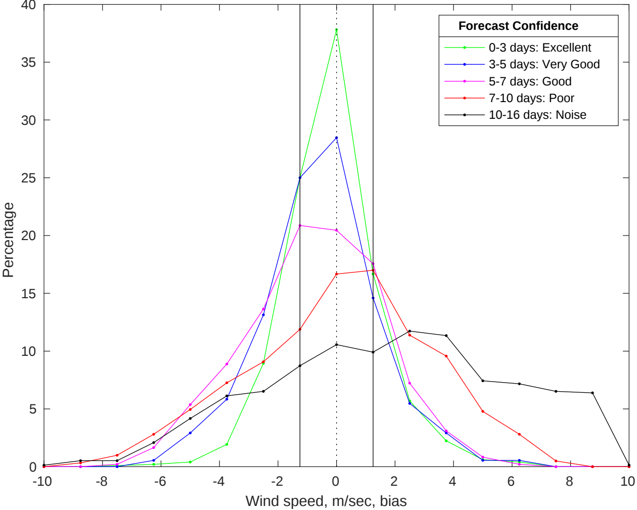
NDBC 46059 vs GFS Winds Bias Histogram: 20-Jan-2026
