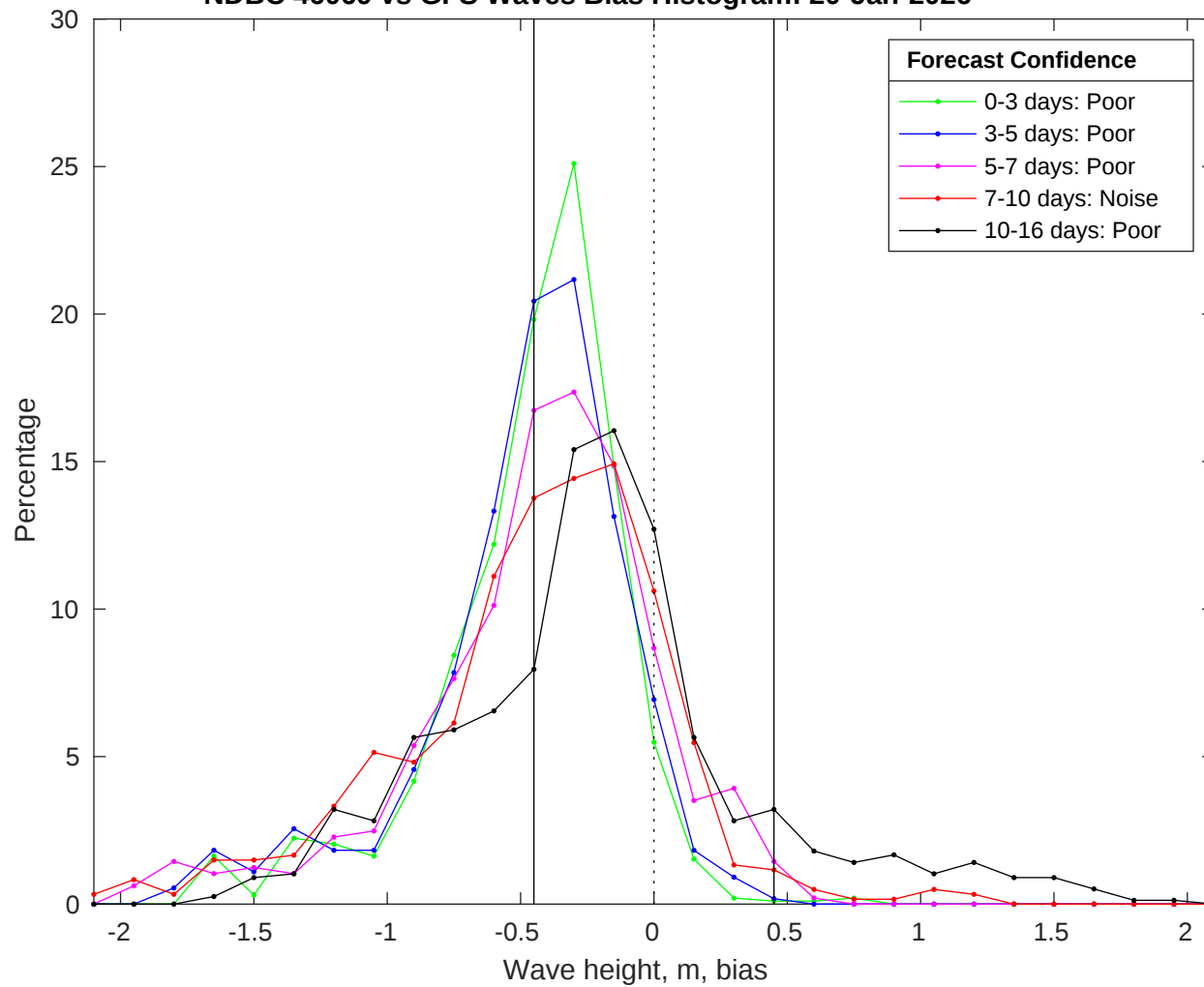
NDBC 46069 vs GFS Waves Bias Histogram: 20-Jan-2026
