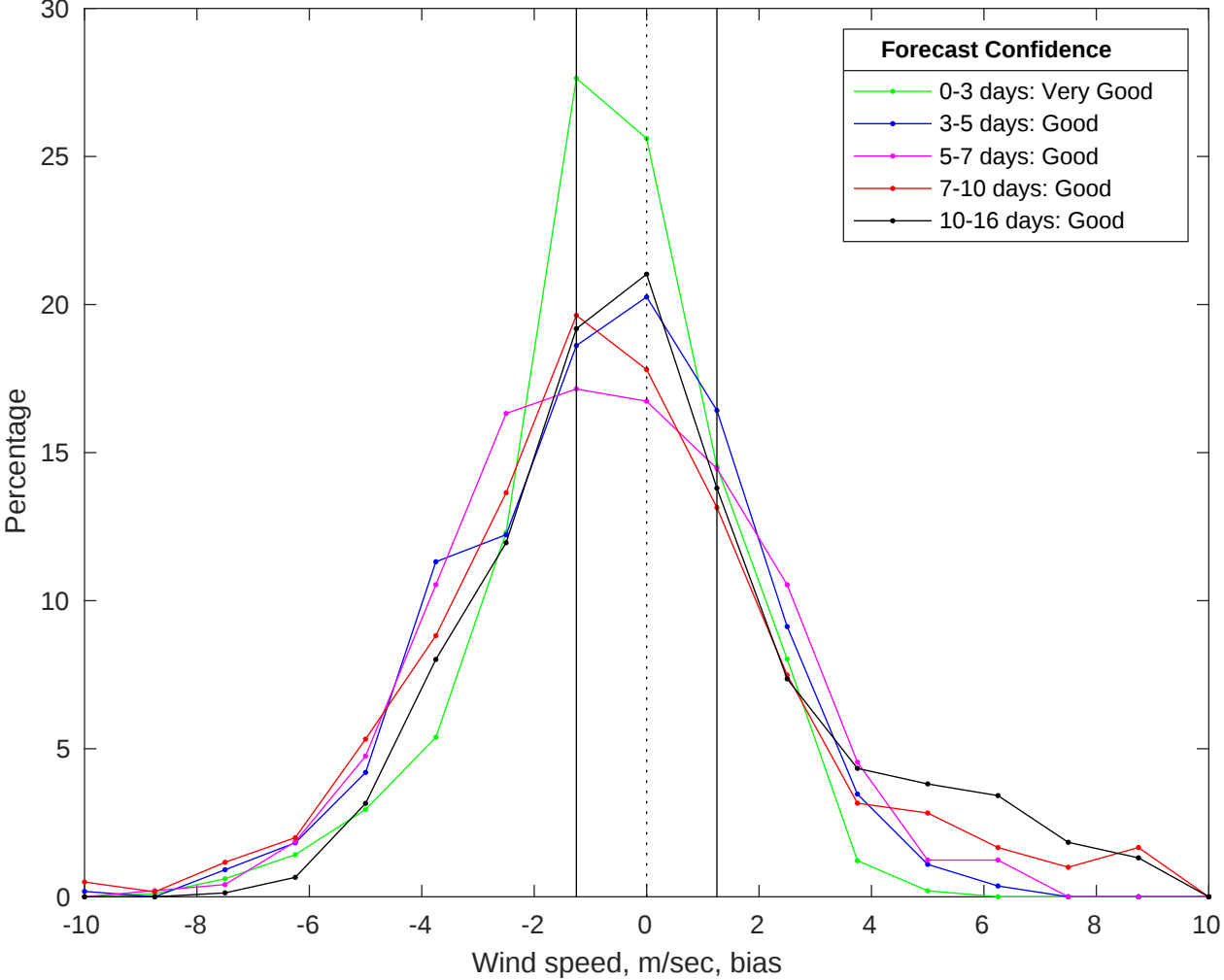
NDBC 46069 vs GFS Winds Bias Histogram: 20-Jan-2026
