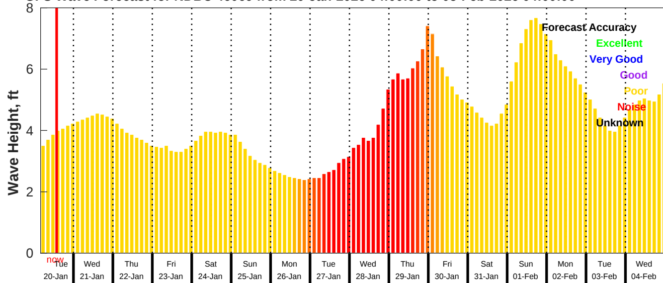
GFS Wave Forecast for NDBC 46069 from 20-Jan-2026 04:00:00 to 05-Feb-2026 04:00:00
