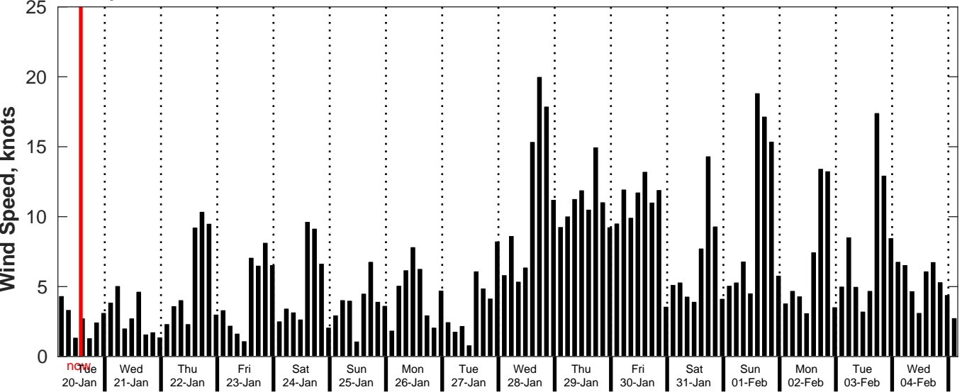
GFS Wind Speed Forecast for NDBC 46215 from 20-Jan-2026 04:00:00 to 05-Feb-2026 04:00:00
