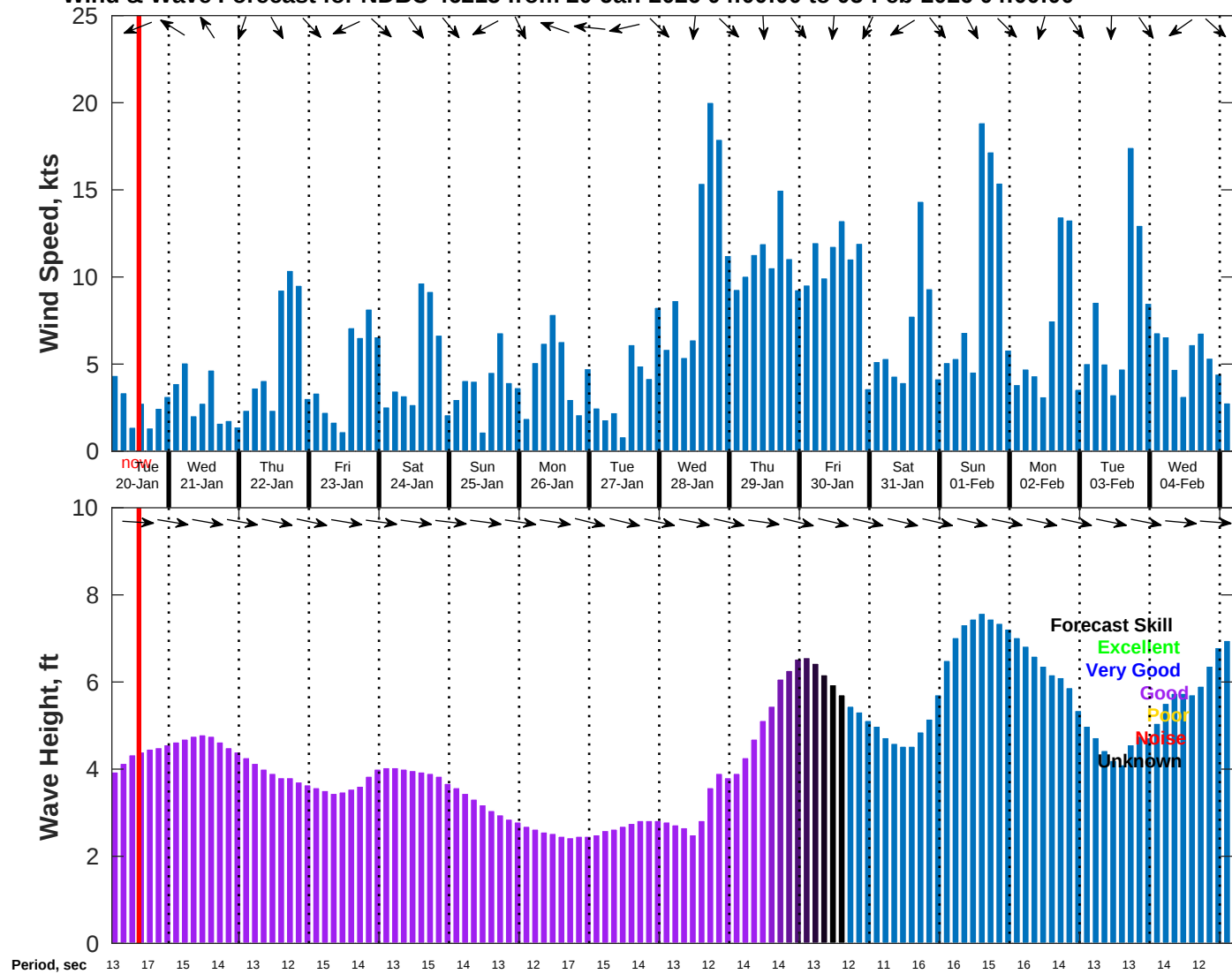
Wind & Wave Forecast for NDBC 46215 from 20-Jan-2026 04:00:00 to 05-Feb-2026 04:00:00
