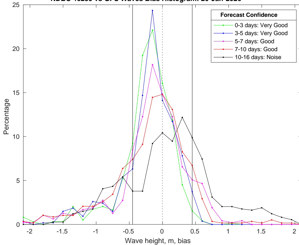
NDBC 46259 vs GFS Waves Bias Histogram: 20-Jan-2026
