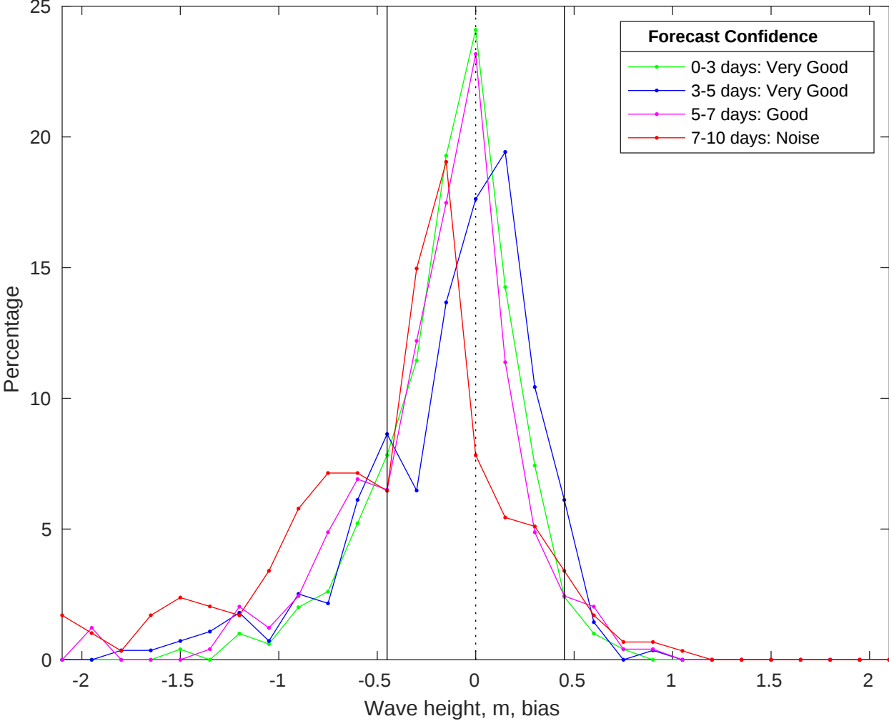
NDBC 51000 vs CMEMS Waves Bias Histogram: 20-Jan-2026
