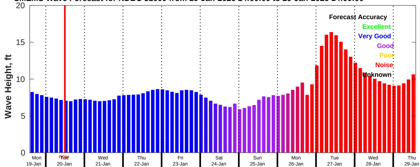
CMEMS Wave Forecast for NDBC 51000 from 19-Jan-2026 14:00:00 to 29-Jan-2026 14:00:00
