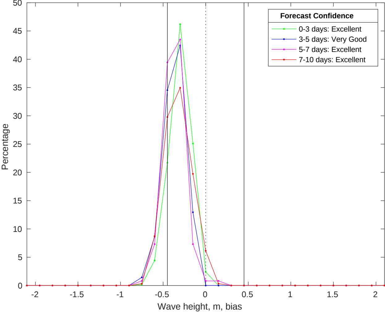
NDBC 51209 vs CMEMS Waves Bias Histogram: 20-Jan-2026
