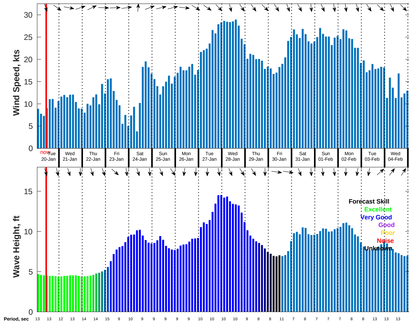
Wind & Wave Forecast for NDBC 51209 from 20-Jan-2026 01:00:00 to 05-Feb-2026 01:00:00
