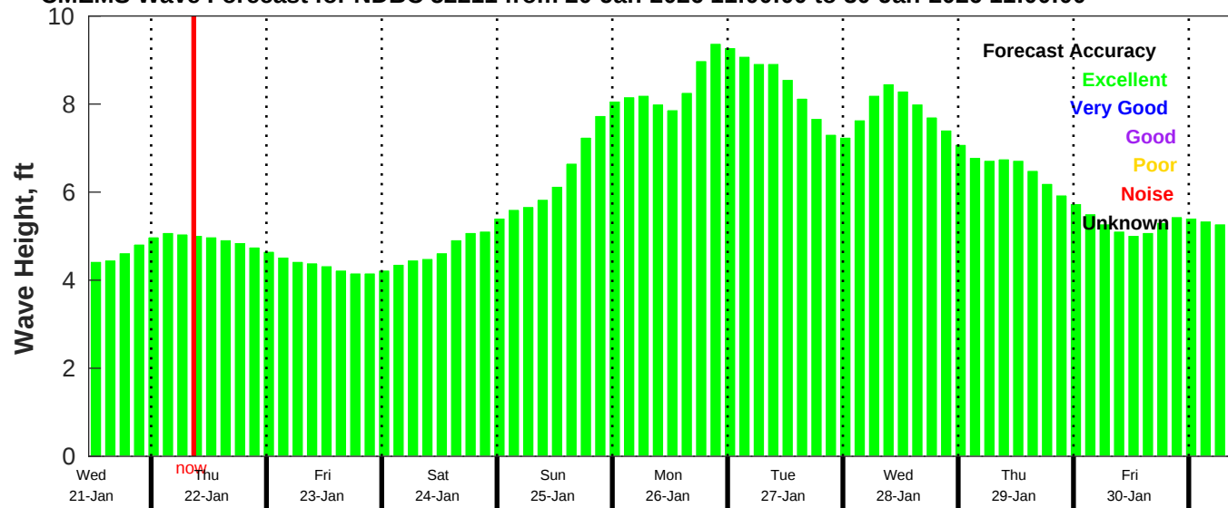
CMEMS Wave Forecast for NDBC 52211 from 20-Jan-2026 11:00:00 to 30-Jan-2026 11:00:00
