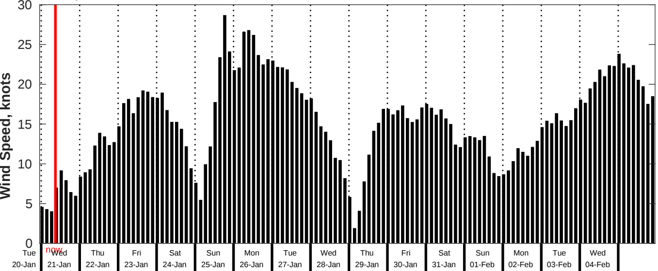
GFS Wind Speed Forecast for NDBC 52211 from 20-Jan-2026 23:00:00 to 05-Feb-2026 23:00:00
