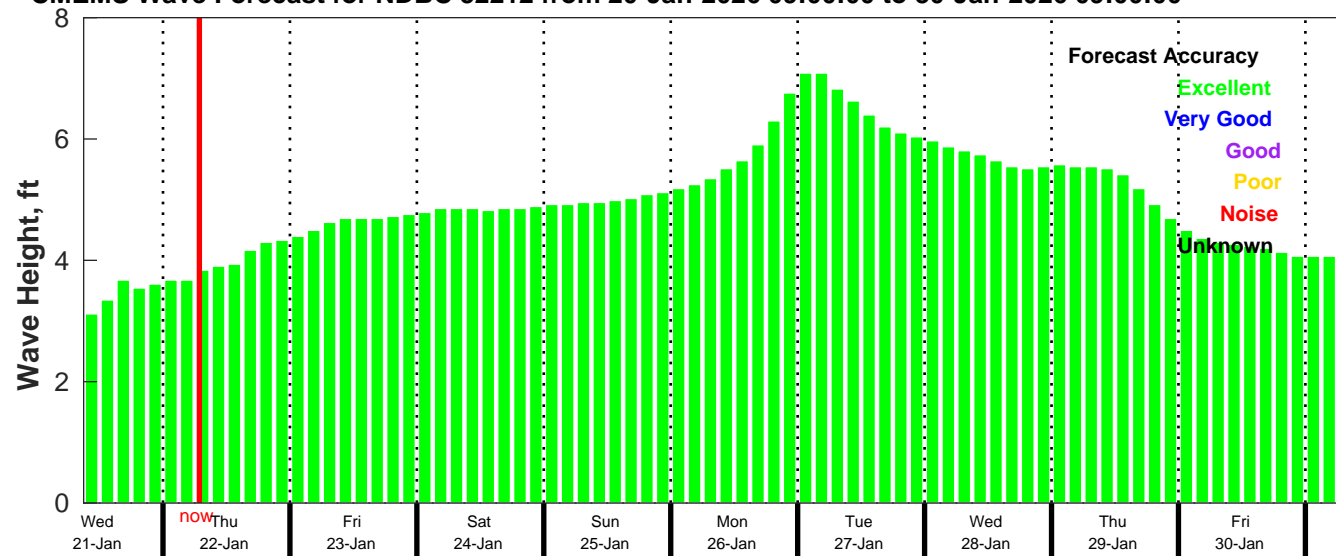
CMEMS Wave Forecast for NDBC 52212 from 20-Jan-2026 09:00:00 to 30-Jan-2026 09:00:00
