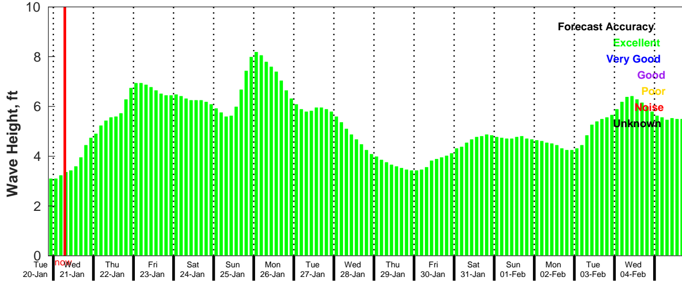
GFS Wave Forecast for NDBC 52212 from 20-Jan-2026 21:00:00 to 05-Feb-2026 21:00:00
