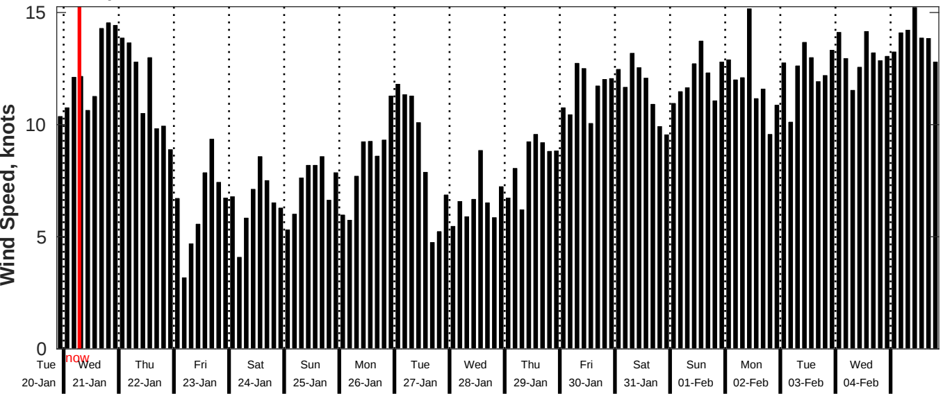
GFS Wind Speed Forecast for NDBC 52212 from 20-Jan-2026 21:00:00 to 05-Feb-2026 21:00:00
