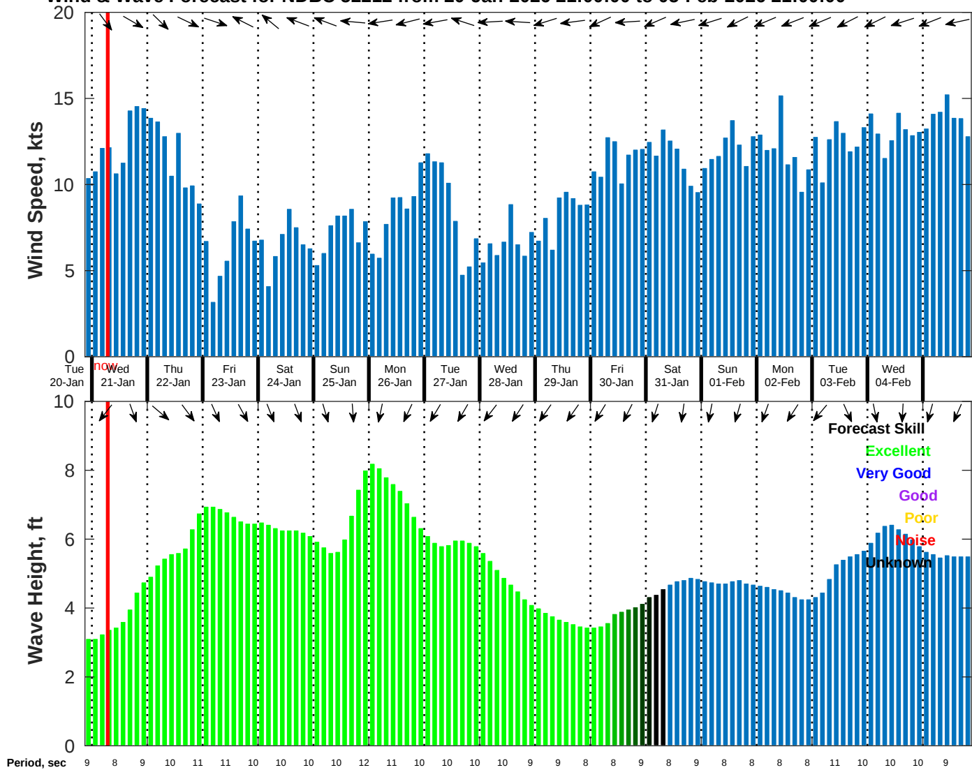
Wind & Wave Forecast for NDBC 52212 from 20-Jan-2026 21:00:00 to 05-Feb-2026 21:00:00
