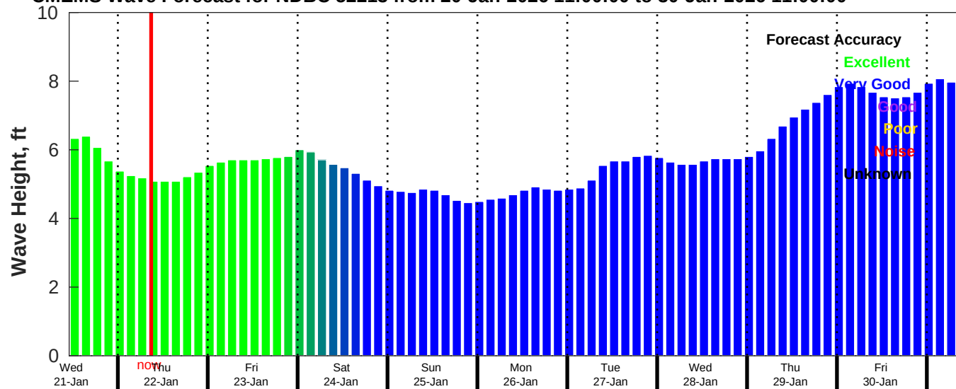
CMEMS Wave Forecast for NDBC 52213 from 20-Jan-2026 11:00:00 to 30-Jan-2026 11:00:00
