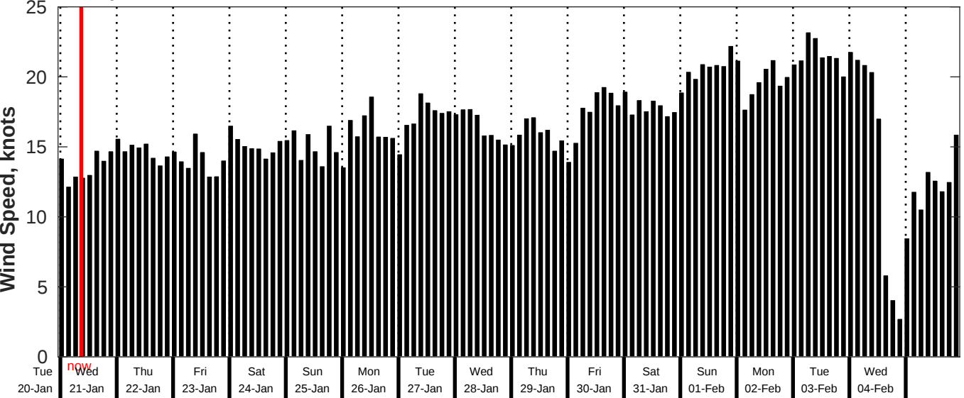
GFS Wind Speed Forecast for NDBC 52213 from 20-Jan-2026 23:00:00 to 05-Feb-2026 23:00:00
