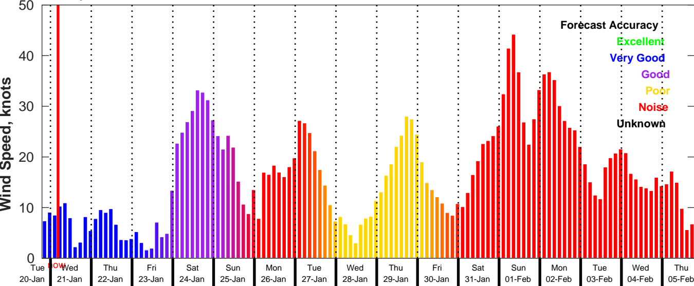
GFS Wind Speed Forecast for NDBC 41004 from 20-Jan-2026 19:00:00 to 05-Feb-2026 19:00:00
