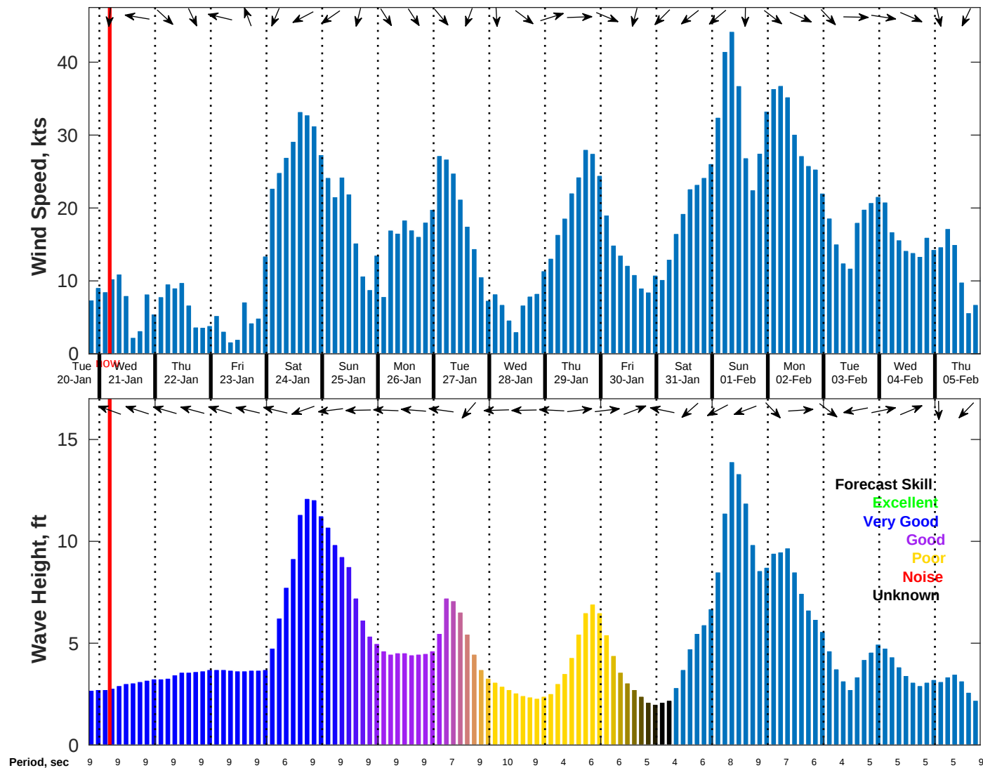
Wind & Wave Forecast for NDBC 41004 from 20-Jan-2026 19:00:00 to 05-Feb-2026 19:00:00
