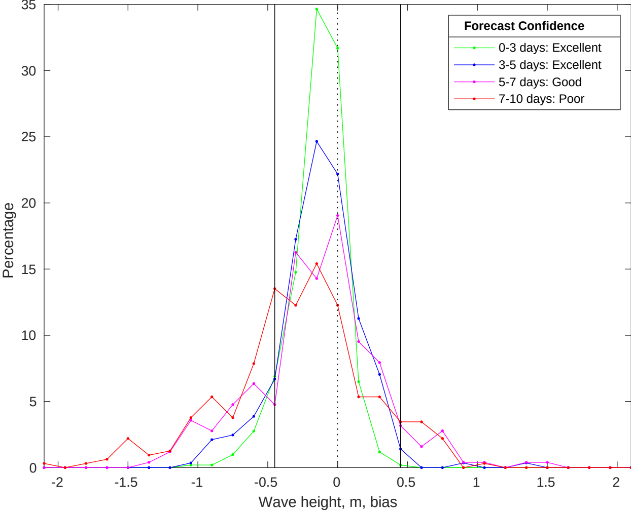
NDBC 41013 vs CMEMS Waves Bias Histogram: 21-Jan-2026
