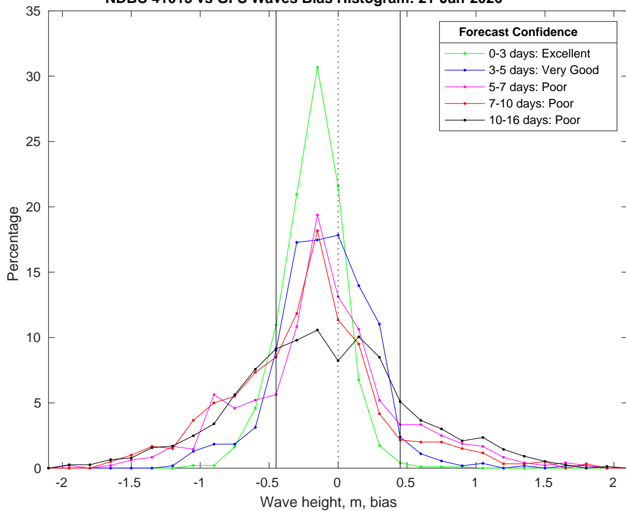
NDBC 41013 vs GFS Waves Bias Histogram: 21-Jan-2026
