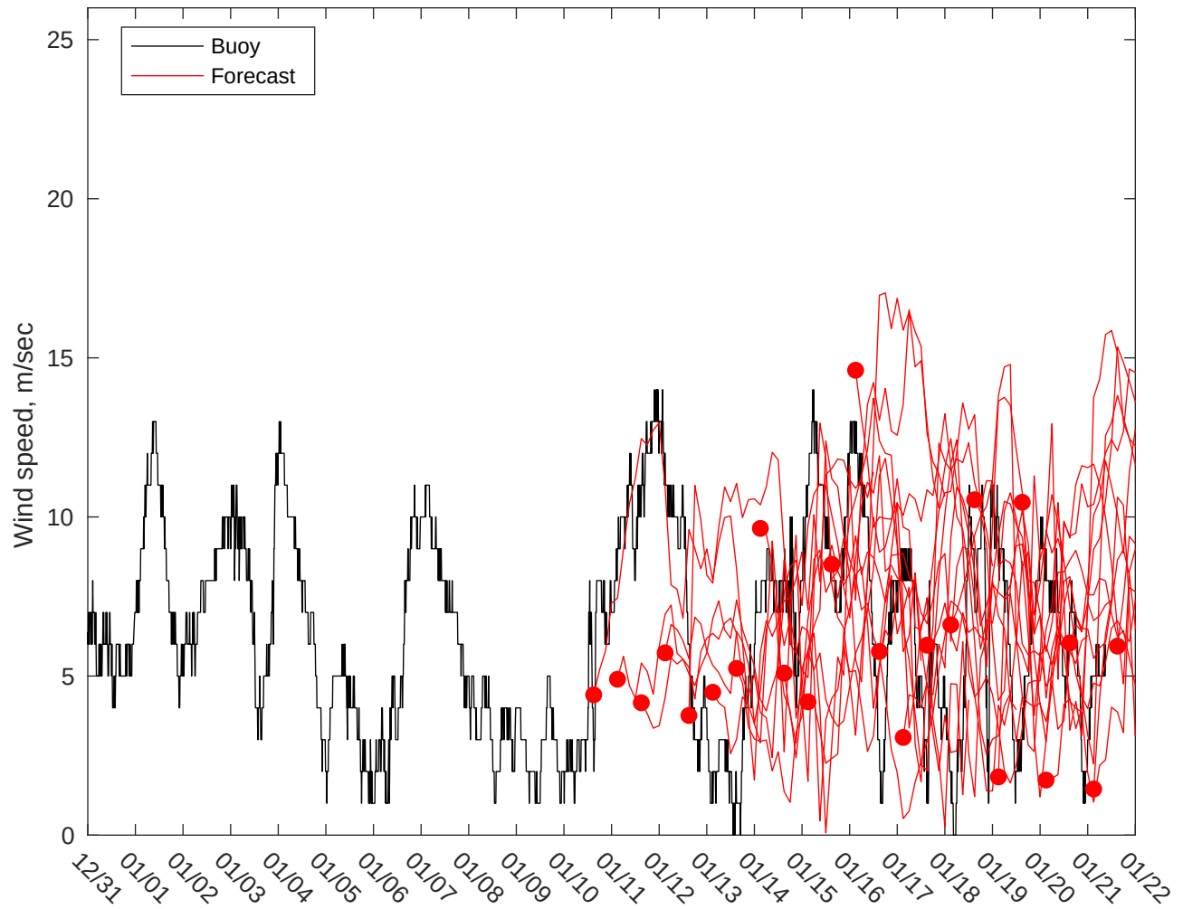
NDBC 41013 vs GFS Winds: 10 to 16 day forecast
