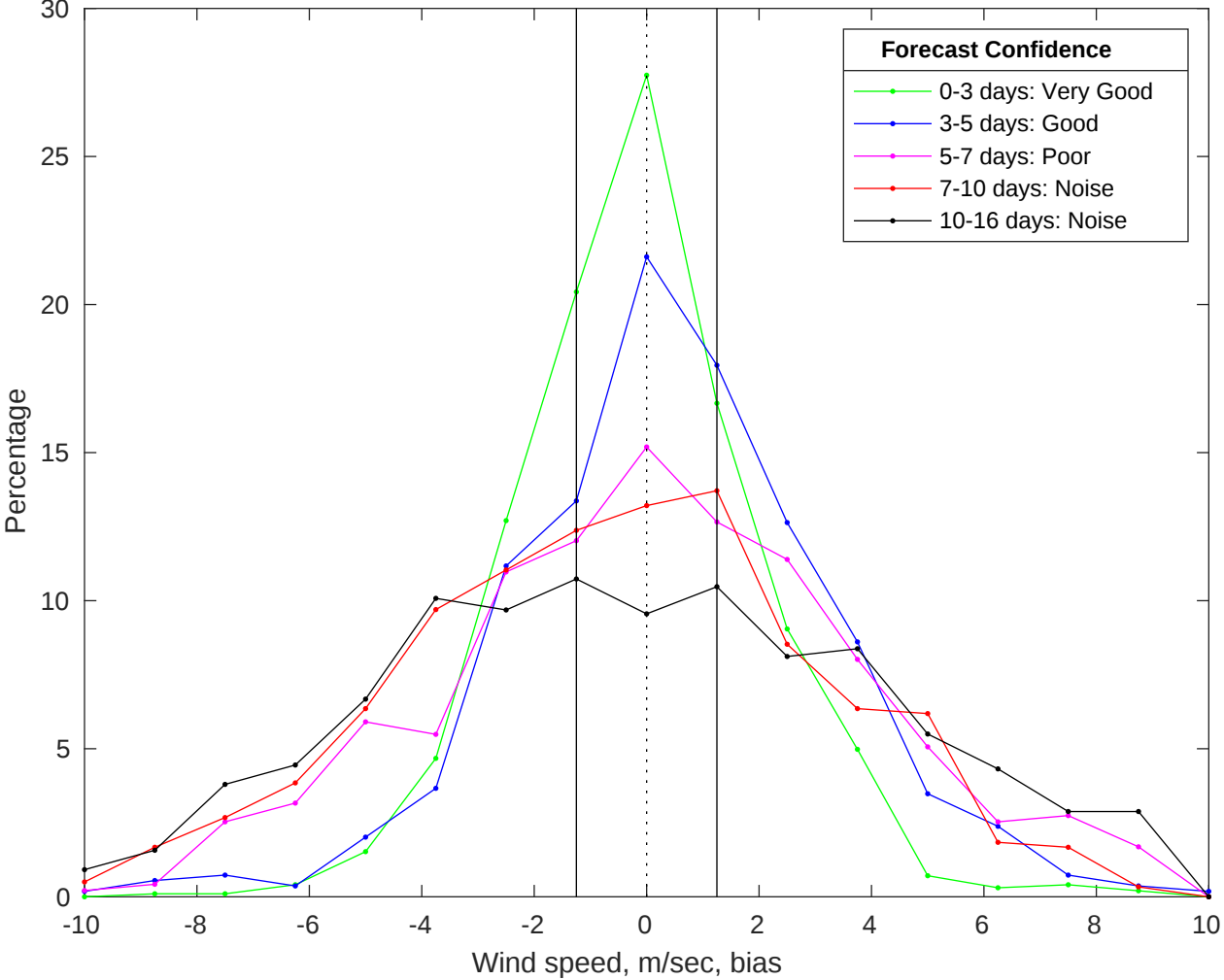
NDBC 41013 vs GFS Winds Bias Histogram: 21-Jan-2026
