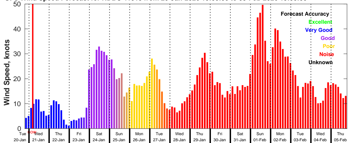
GFS Wind Speed Forecast for NDBC 41013 from 20-Jan-2026 19:00:00 to 05-Feb-2026 19:00:00
