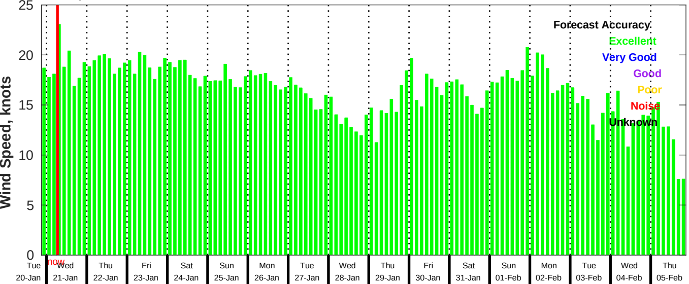
GFS Wind Speed Forecast for NDBC 41040 from 20-Jan-2026 21:00:00 to 05-Feb-2026 21:00:00
