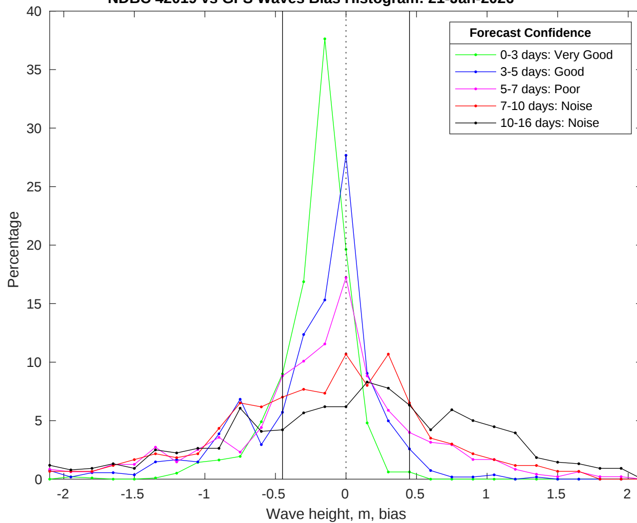
NDBC 42019 vs GFS Waves Bias Histogram: 21-Jan-2026
